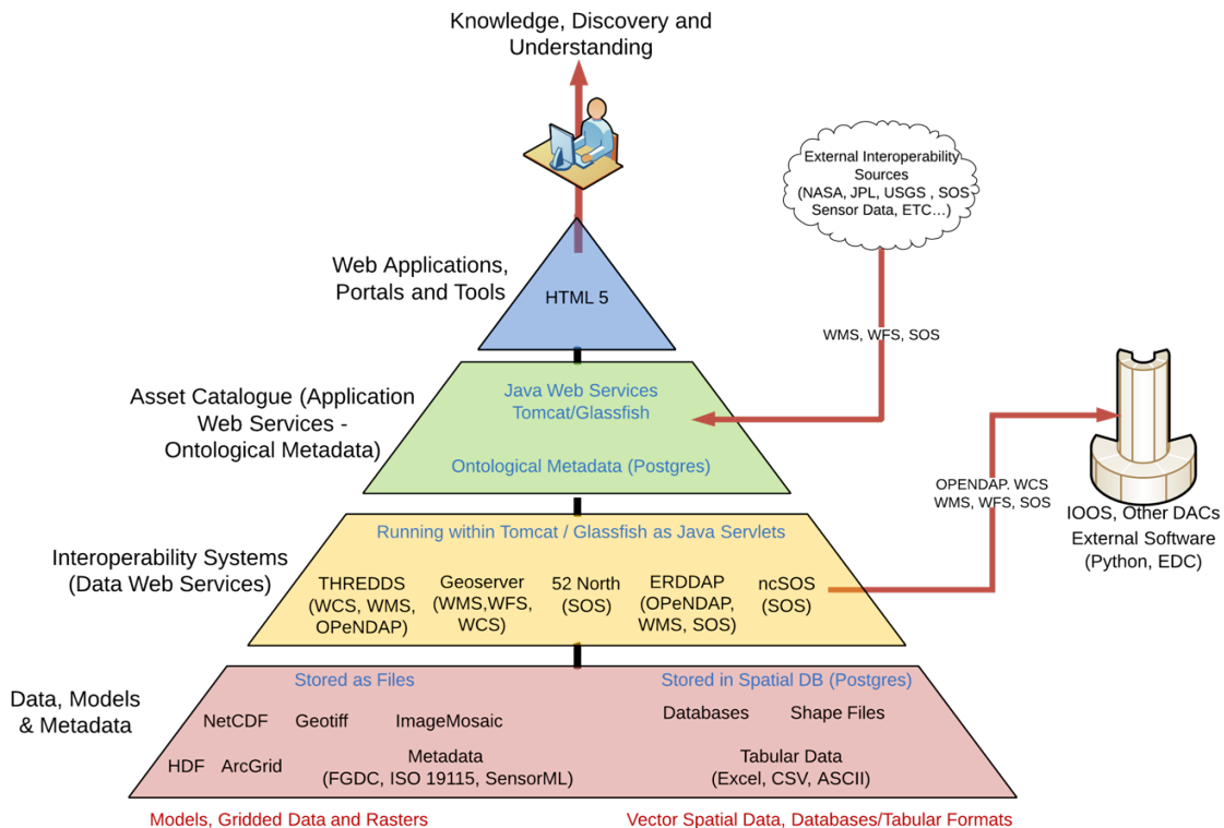
Figure 2. A schematic of the AOOOS Data System that details the flow of data through logical technology tiers so that it can be consumed by users to enable discovery and understanding of EVOSTC-funded data and products.
