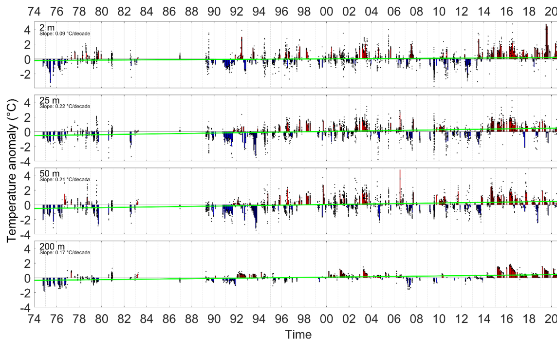
Figure 1. Temperature anomalies at four selected depths in central Prince William Sound. Anomalies were calculated as the residual to a second order cosine curve fit to all years data (to remove seasonality: Campbell 2018). Black points are observations, bars are biweekly averages, and the green line indicates the linear trend. All slopes were significantly different from zero ( p < 0.05 ).
