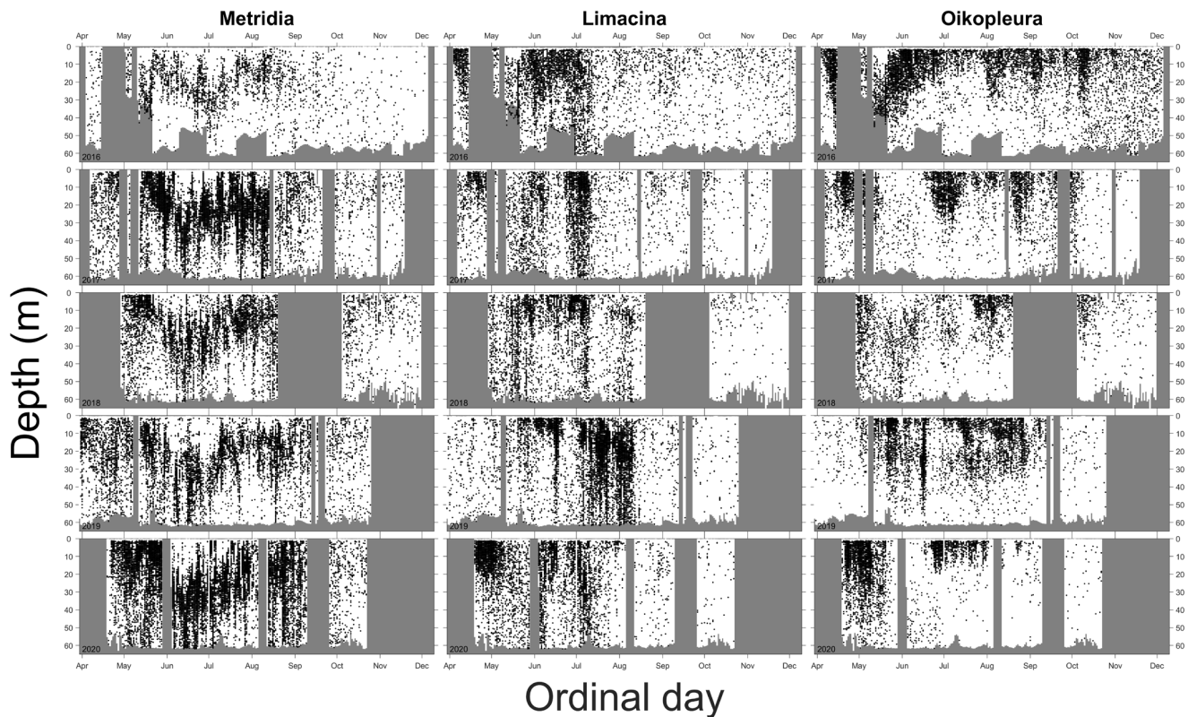
Figure 5. Time-depth distributions of individual plankters of three of the more common large taxa found in the Prince William Sound plankton ecosystem (column-wise: Metridia sp., Limacina helacina , and Oikopleura sp.) in each year of deployments (row-wise with 2016 at the top and 2020 at the bottom). Each point represents an image that was classified as being of an individual plankter of the species. Each image was time-stamped (nearest millisecond) when collected and the depth then determined from the time-pressure record of the CTD on the profiler.
