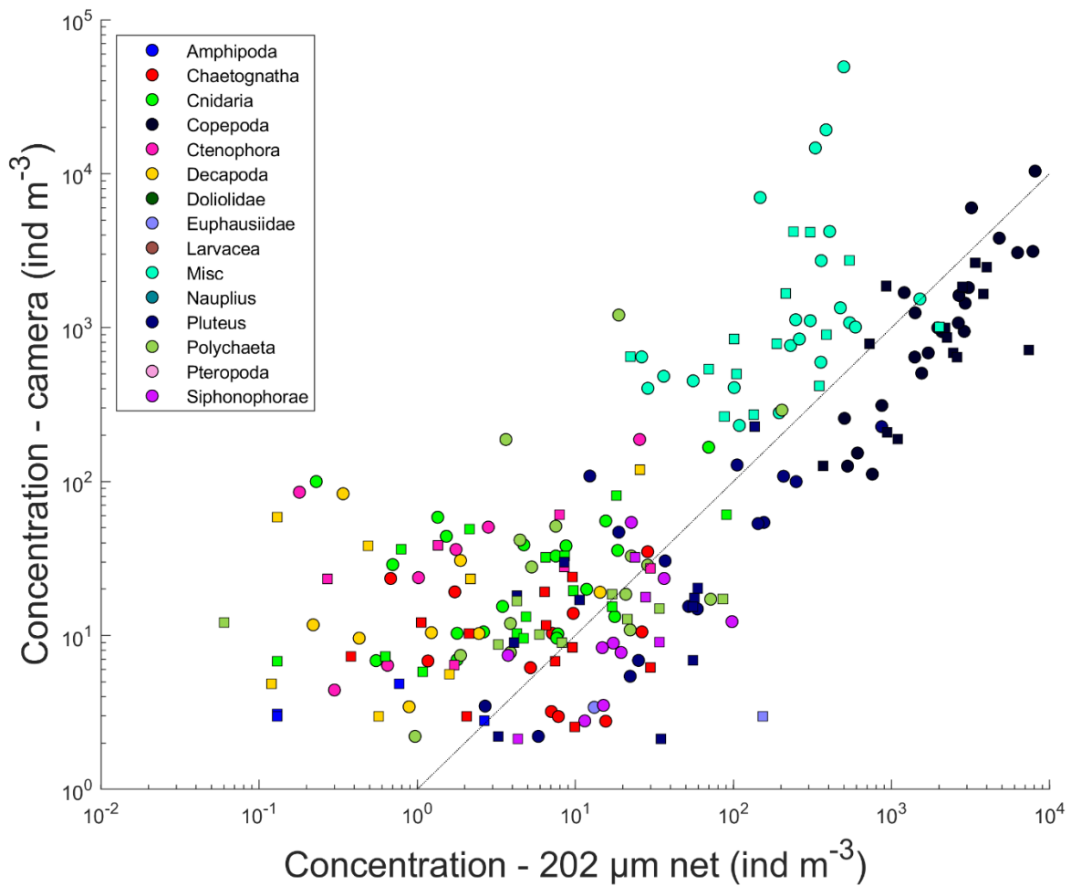
Figure 4. Comparison of abundance estimates derived from the plankton camera aboard the Prince William Sound Profiler (ordinate) and a 202 µm plankton net, by various taxa groups. The dashed line indicates the 1:1 line. Plankton tows were done after profiler service visits, and the tow was done from 0-60 m (the depth that the profiler samples), and as close in time to a profile as possible (usually <1 hour).
