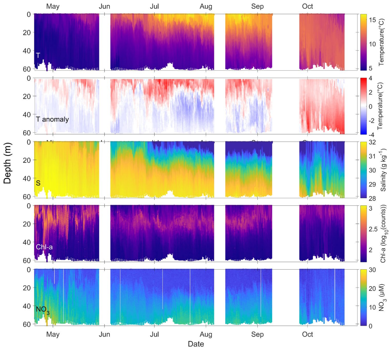
Figure 3. Time series of observations made by the Prince William Sound autonomous profiler in 2019. Top panel: temperature ( ^{\circ}\text{C} ). Second panel: Temperature anomaly ( ^{\circ}\text{C} ). Temperature anomalies were calculated with the method of Campbell (2018) used in Fig. 1. Third panel: Salinity (TEOS-10). Fourth panel: Chlorophyll-a fluorescence. Chlorophyll is presented as \log_{10} transformed digital counts (counts are linearly proportional to chlorophyll-a concentration). Fifth panel: Nitrate concentration ( \mu\text{M} ) from a Satlantic SUNA.
