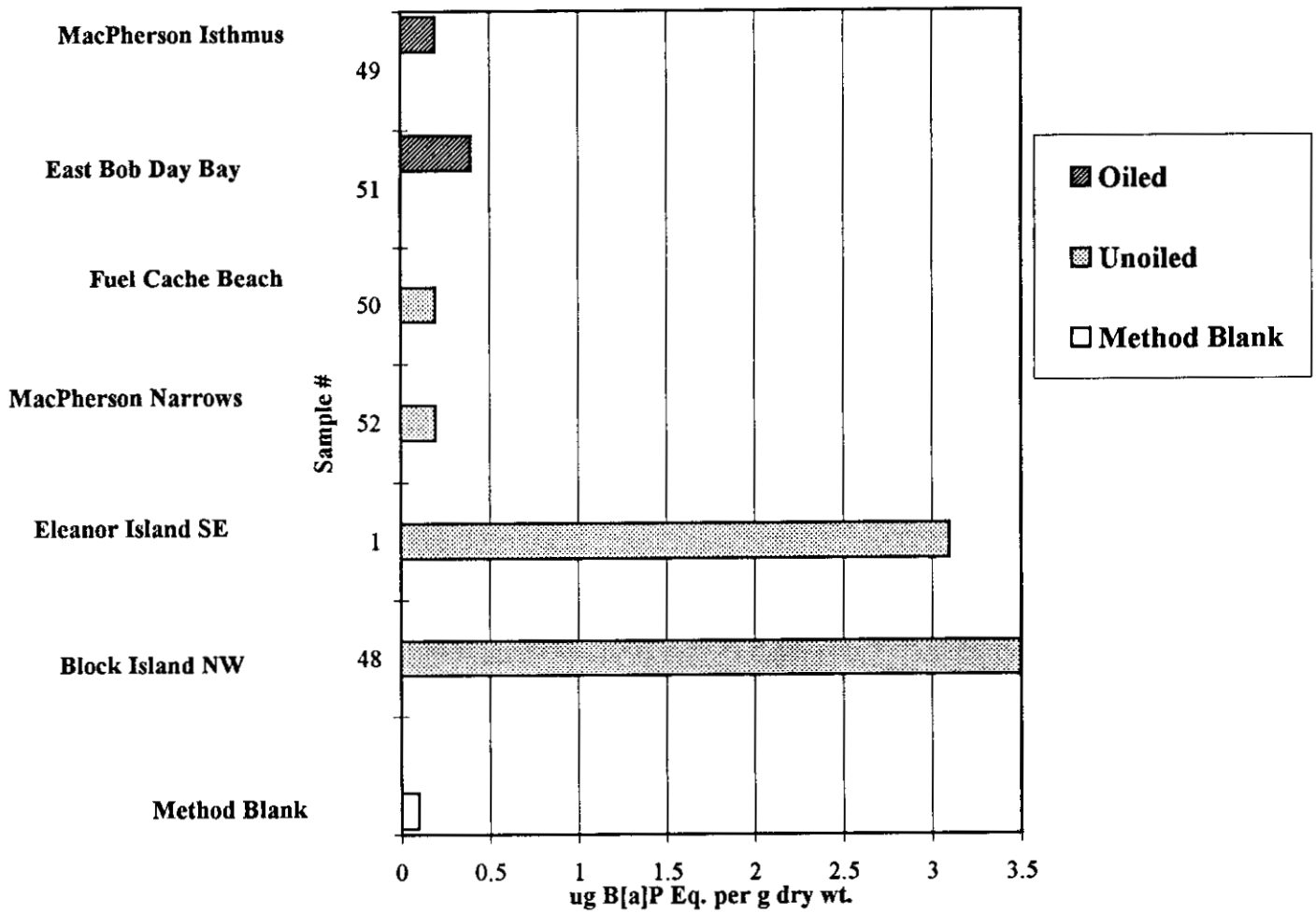
Figure 2. P450 RGS-estimated B[a]P Equivalents in Sediments from Prince William Sound, Alaska
