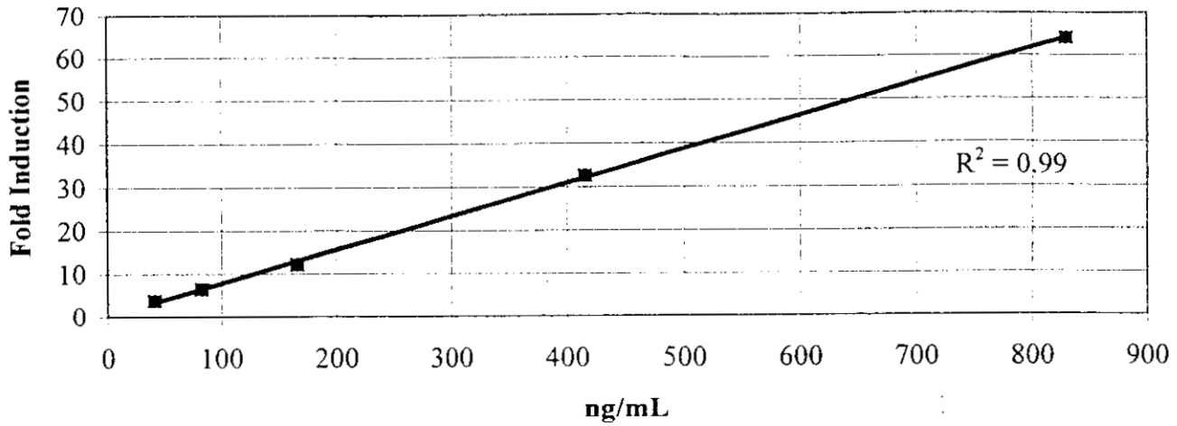
Figure 6. Luciferase Standard Curve (11/6/96)
