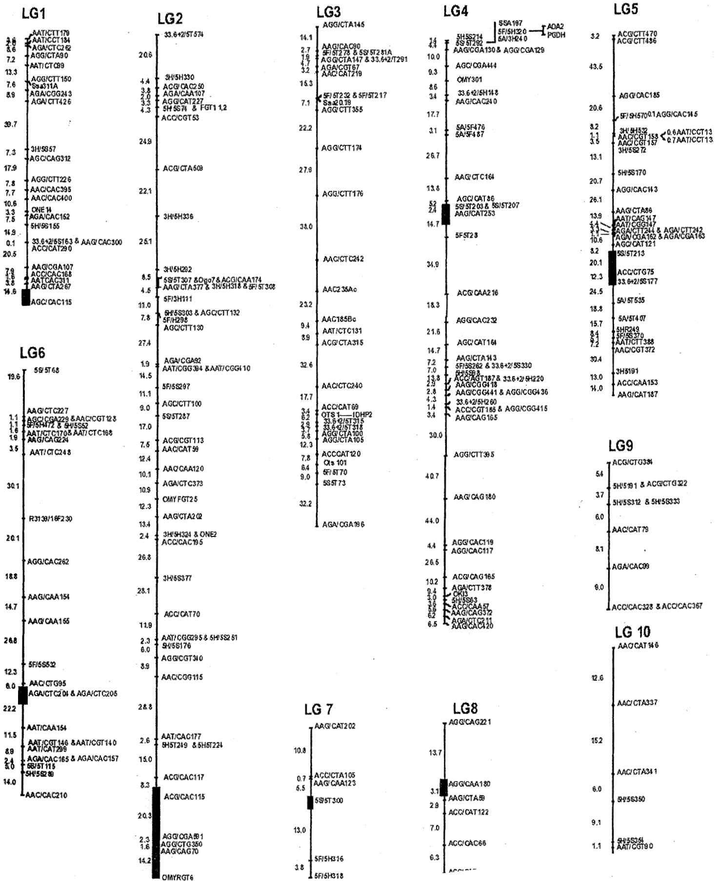
Figure 1. Genetic linkage map of pink salmon based on the inheritance of 602 polymorphic loci. Numbers to the left indicate recombination rates (cM). Locus names are to the right. Centromeres are indicated by black rectangles.
