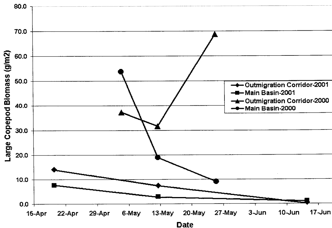
Figure 7. Comparison of large copepod biomass estimates for the out-migration corridor and main basin during 2000 and 2001 surveys.
