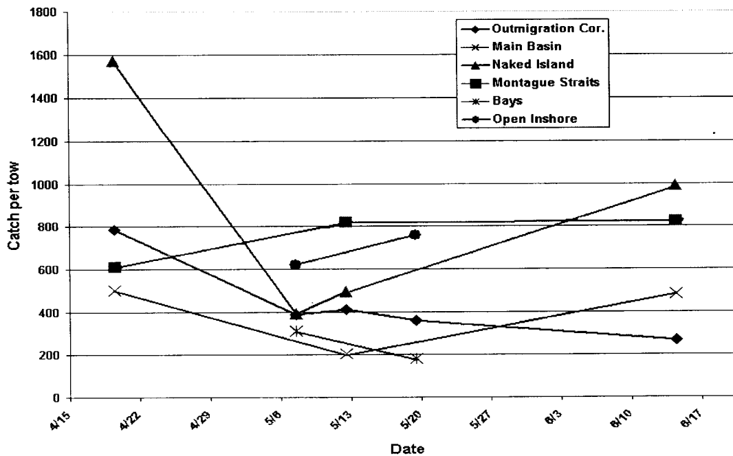
Figure 3. Catches of large copepods by cruise date and location
