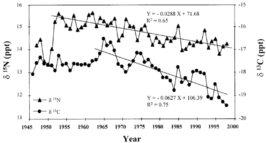
Figure 1. Inter-decadal shift in ^{15}\text{N}/^{14}\text{N} and ^{13}\text{C}/^{12}\text{C} content (vertical axis) of bowhead whale baleen ascribed to feeding in the Bering Sea; from Schell (2001).
