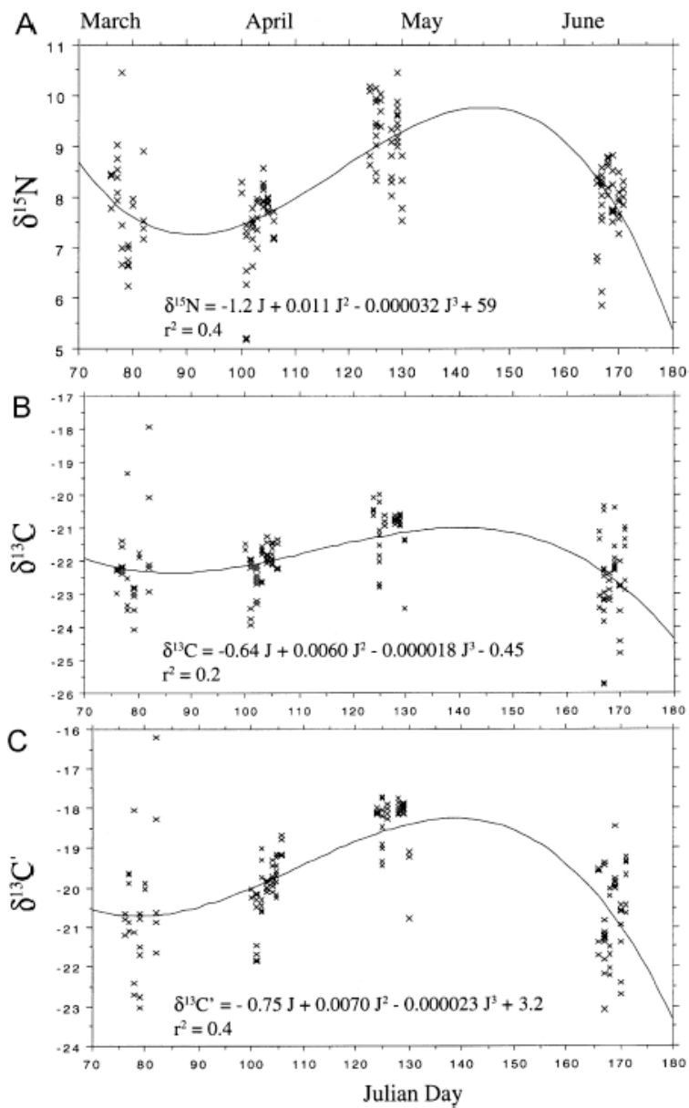
Figure 2. Seasonal shifts in the in ^{15}\text{N}/^{14}\text{N} (A) and ^{13}\text{C}/^{12}\text{C} (B (raw data) & C (lipid-normalized)) content (vertical axis) of bulk net zooplankton collected during March to June 1995 (Julian Day = Day of the Year) in the northern Gulf of Alaska and Prince William Sound, from Kline (1999). Panels B and C reflect increase in correlation resulting from correction for lipid content.
