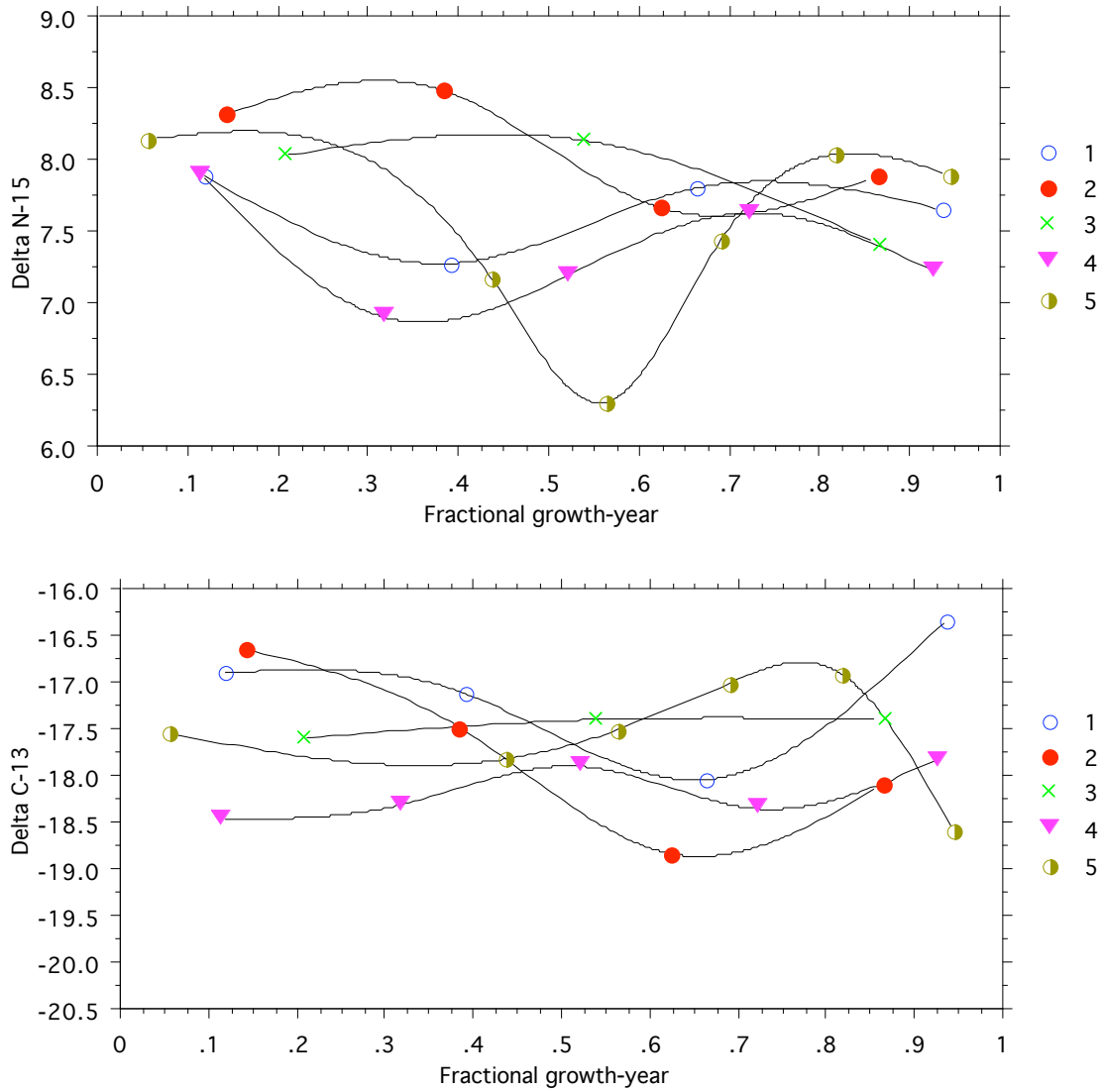
Figure 4. Fractional growth-year isotopic patterns. \delta^{15}\text{N} and \delta^{13}\text{C} values of Mytilus californianus periostracum samples, for individual animals A to C, in relation to apparent annual growth patterns. Values near 0 reflect early growth while values near 1, reflect growth just prior to an annulus. 1,2 ,and 3 of Mytilus ‘A’ corresponded to 1990, 1989, and 1988; 1,2 , 3, and 4 of Mytilus ‘B’ corresponded to 1989, 1987, and 1986, while 1, 2, 3, 4, and 5 of Mytilus ‘C’ corresponded to 1985, 1984, 1983, 1982, and 1981.
