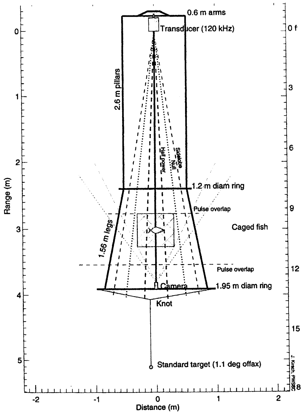
Figure 1. Side view of experimental frame used for target strength measurements showing locations of transducer, fish, camera and standard target.
