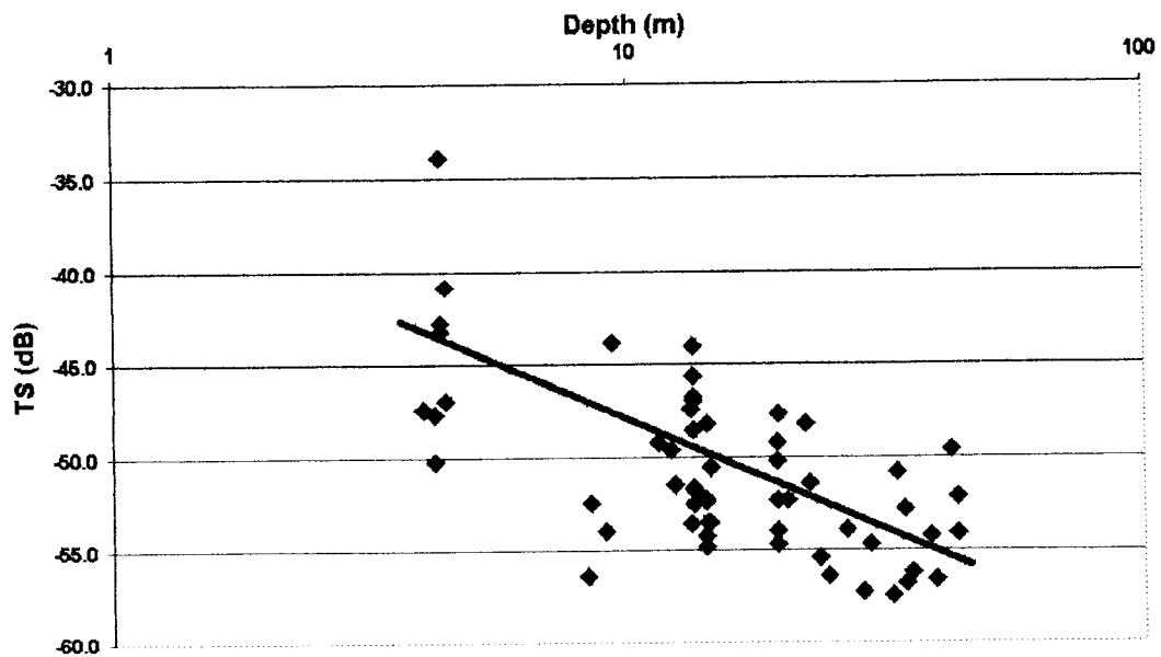
Figure 3. Scatter plot of Pacific herring target strengths at various depths.
