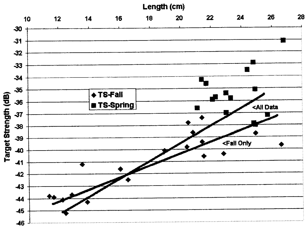
Figure 2. Observed target strength (dB) to length relationship of Pacific herring.
