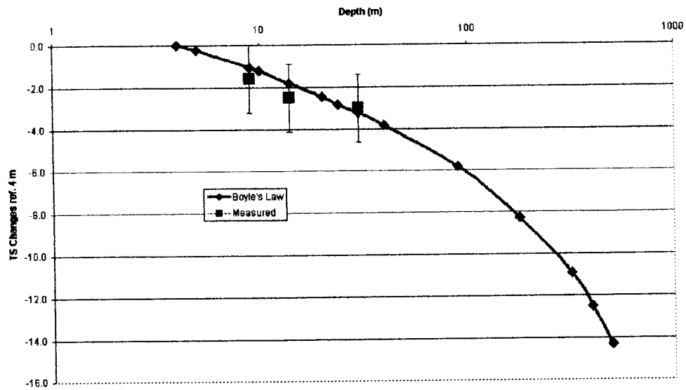
Figure 4. Comparison of observed changes in target strength with those predicted from Boyle's law, i.e. \Delta TS = -6.7P + 3.17 (Mukai and Iida 1996).
