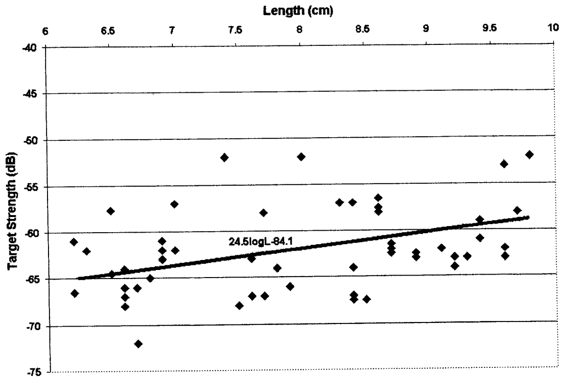
Figure 6. Observed target strength to length relationship for Pacific sand lance.
