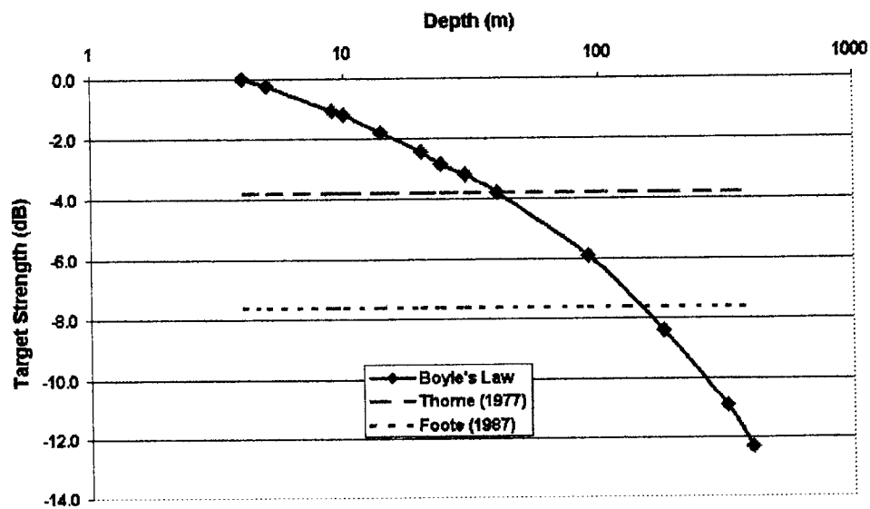
Figure 5. Depth dependent changes in TS compared to depth independent equations of Thorne (1977a) and Foote (1987). The depth dependent function is the target strength measured at 4 m in this study as modified by Boyle's law.
