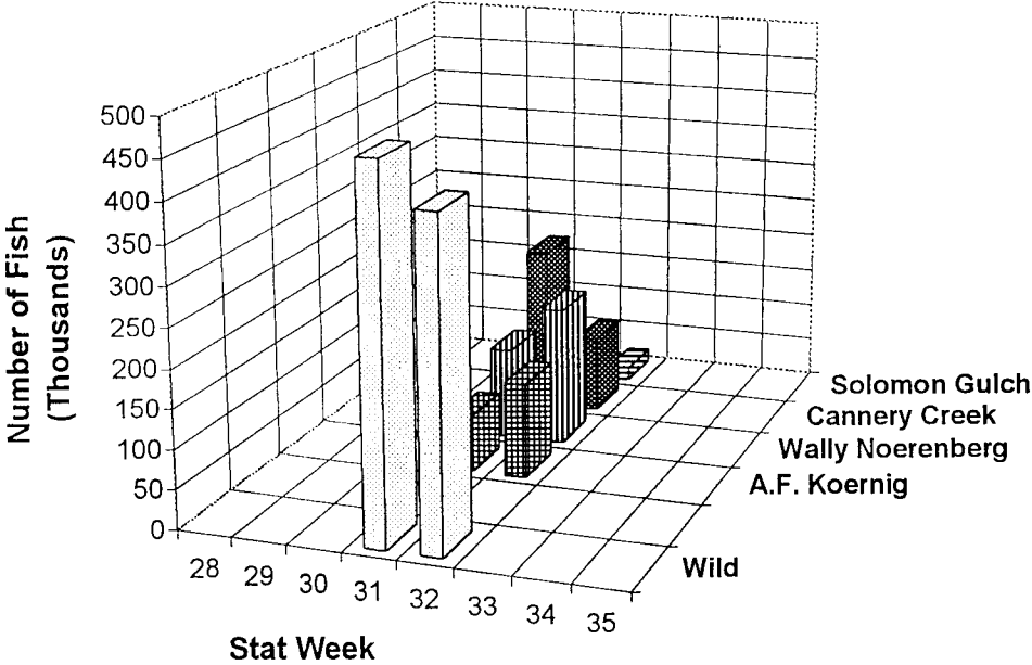
Figure 7 Hatchery and wild stock contributions to Southwestern district common property fishery catches by district and week in Prince William Sound in 1995.
