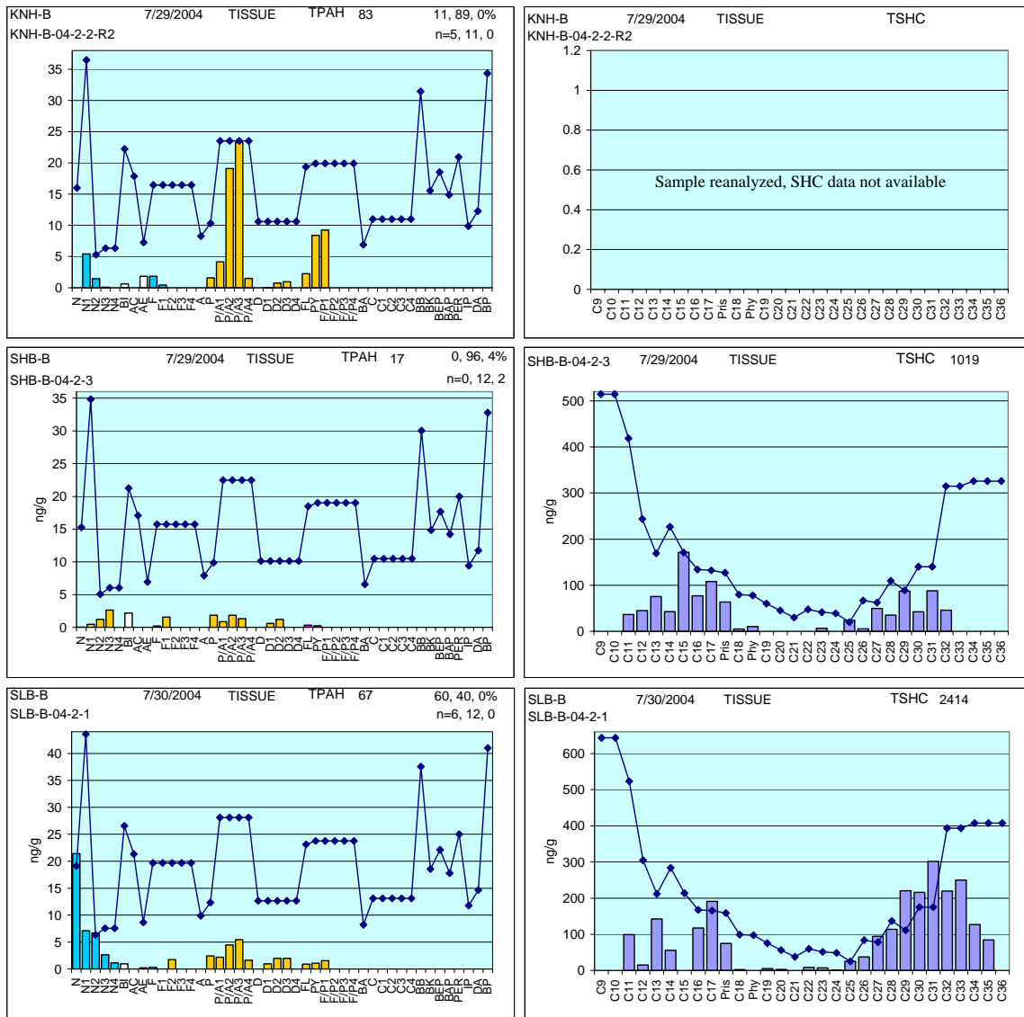
Figure 25 Representative Knowles Head, Sheep Bay and Sleepy Bay Mytilus PAH and SHC profiles showing low-level particulate/oil-phase components in July 2004. MDLs indicated with dotted solid line.
