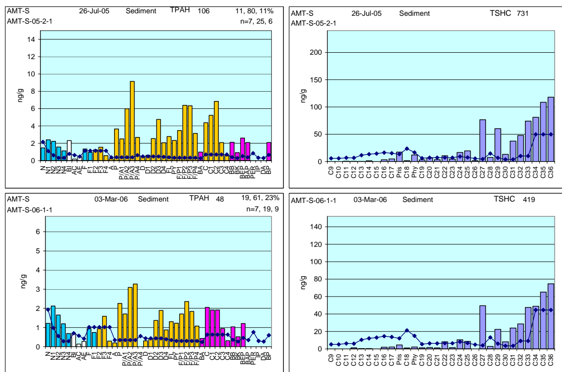
Figure 11 PAH and SHC profiles from representative AMT sediment in July 2005 and March 2006 showing complex, oil/particulate-dominated signatures in a heavily weathered and biodegraded, mixed signal. MDLs indicated with dotted solid line.
