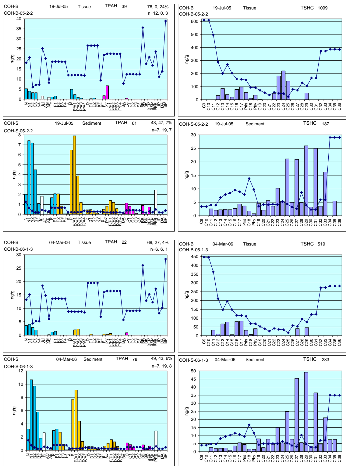
Figure 29 Representative Constantine Harbor Mytilus and adjacent intertidal sediment PAH and SHC profiles from samples collected as part of the EVOS Trustees SCAT program in July 2005 and March 2006. MDLs indicated with dotted solid line.
