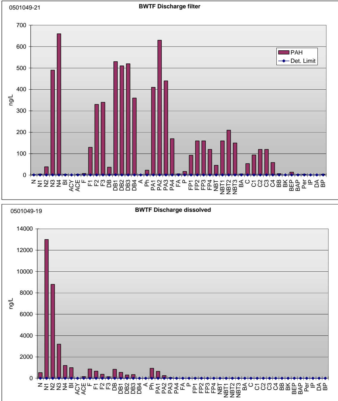
Figure 2 PAH profiles of oil droplets removed by filtration (upper) and the dissolved-phase (lower) of the AMT BWTF effluent, January 2005 (from Payne et al. 2005b).
