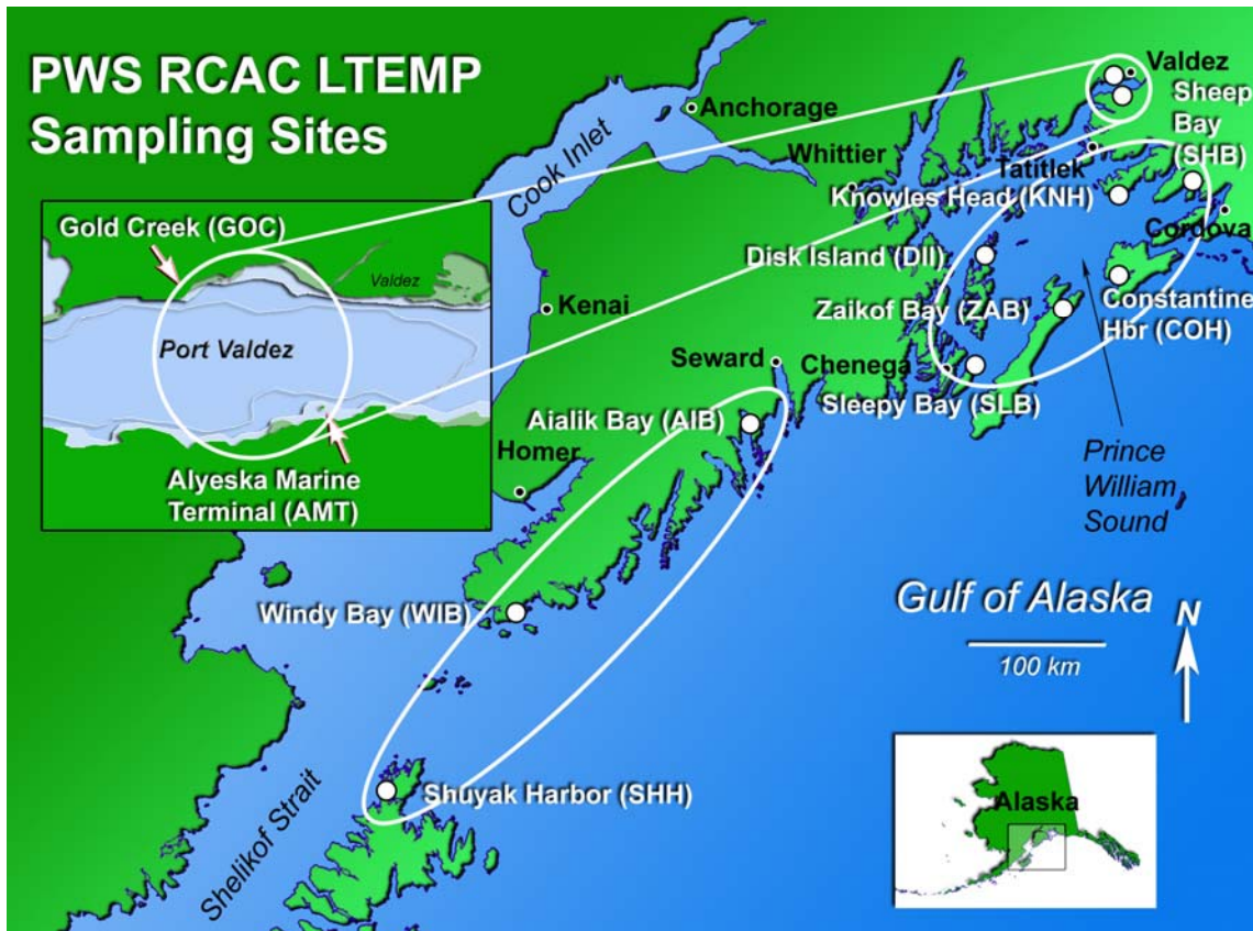
Figure 1 Map of the 2005/2006 LTEMP sites.
