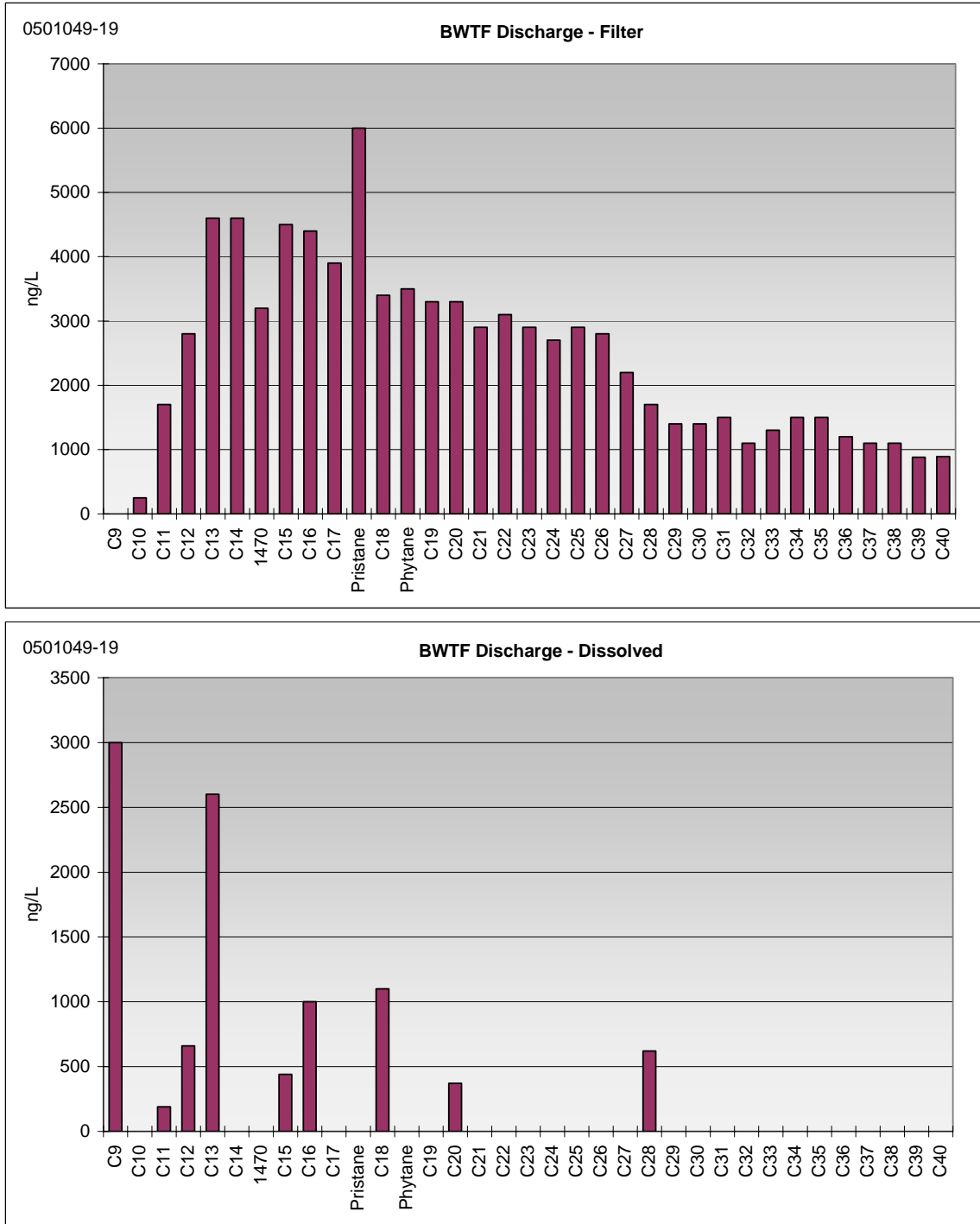
Figure 3 SHC profiles of oil droplets removed by filtration (upper) and the dissolved-phase (lower) of the AMT BWTF effluent, January 2005 (from Payne et al. 2005b).
