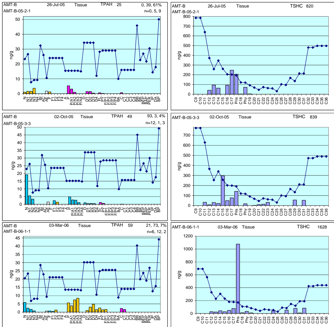
Figure 17 PAH and SHC profiles showing low-level TPAH with variable source signals (combustion-, dissolved-, and oil/particulate-phase) in AMT mussel samples collected in July 2005, October 2005 and March 2006, respectively. MDLs indicated with dotted solid line.
