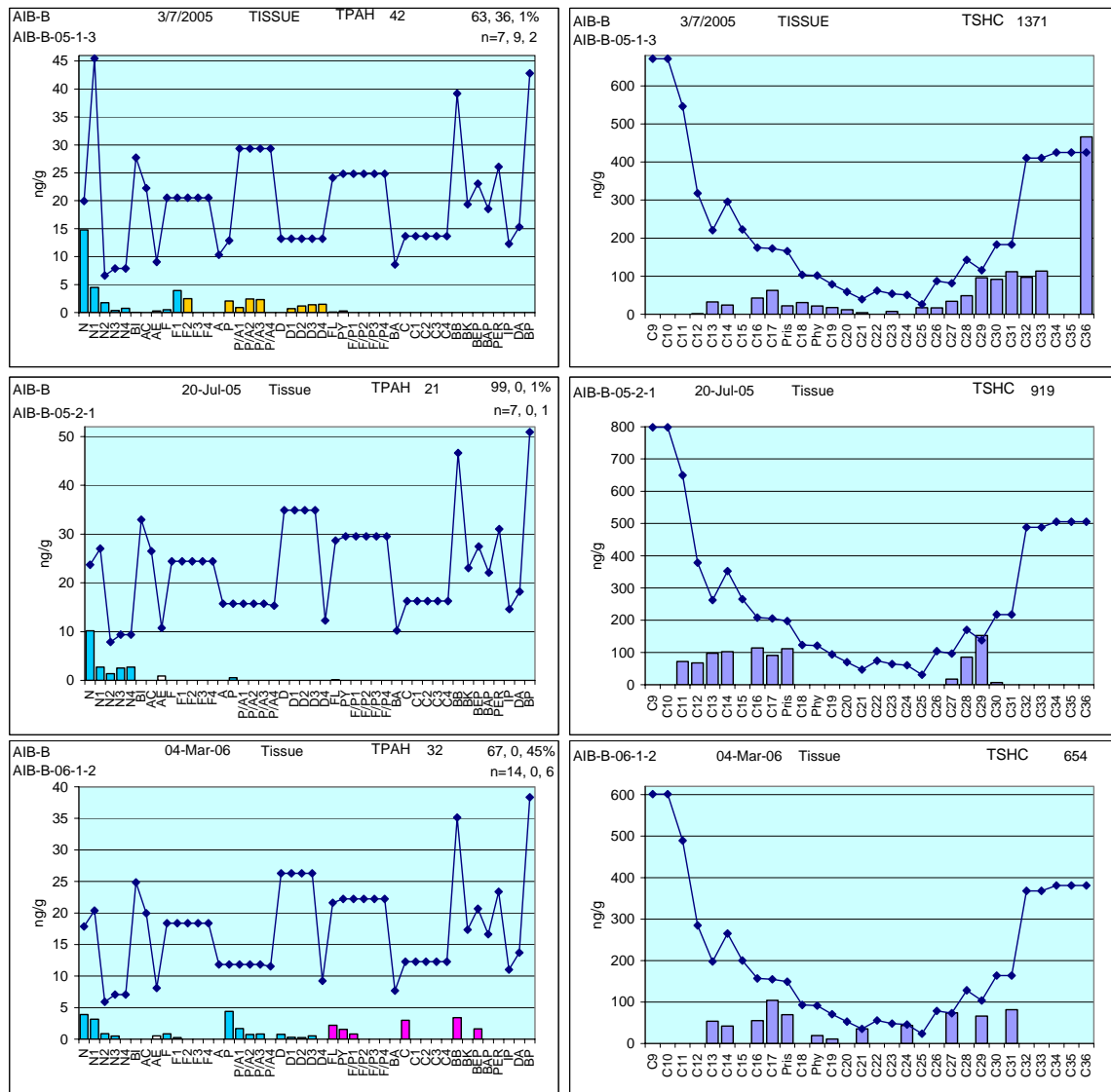
Figure 31 Representative Aialik Bay Mytilus PAH and SHC profiles showing a mixed dissolved- and particulate/oil-phase pattern in March 2005, dissolved-phase components in July 2005, and mixed dissolved- and combustion-phase components in March 2006. The SHC profiles show just-below MDL traces of biogenic and petrogenic components in March 2005, with less-than MDL marine and terrestrial biogenic input in July 2005 and March 2006. MDLs indicated with dotted solid line
