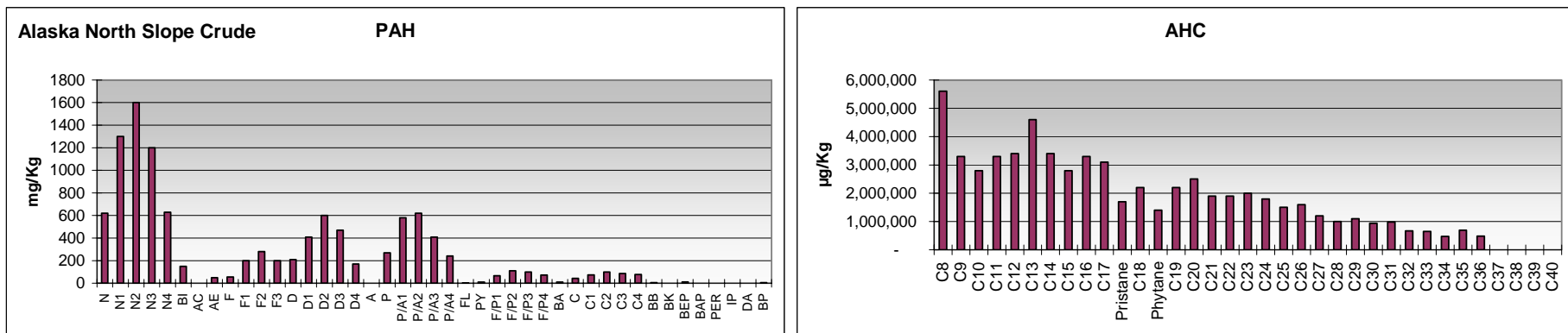
Appendix Figure 1 Example plots of ANS PAH and SHC (also referred to as AHC) components.
