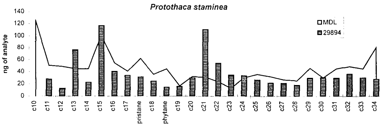
Figure 3. Aliphatic hydrocarbons in representative clams from Green Island. Note that the area under the MDL curve is not a significant factor, rather the points are connected to highlight the MDL.
