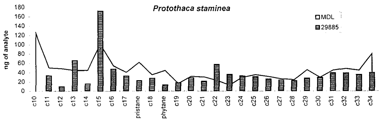
Figure 4. Aliphatic hydrocarbons in representative clams from Montague Island. Note that the area under the MDL curve is not a significant factor, rather the points are connected to highlight the MDL.
