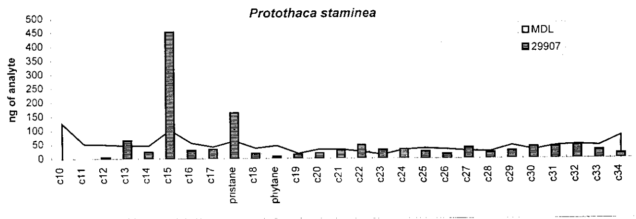
Figure 2. Aliphatic hydrocarbons in representative clams from Squirrel Island. Note that the area under the MDL curve is not a significant factor, rather the points are connected to highlight the MDL.
