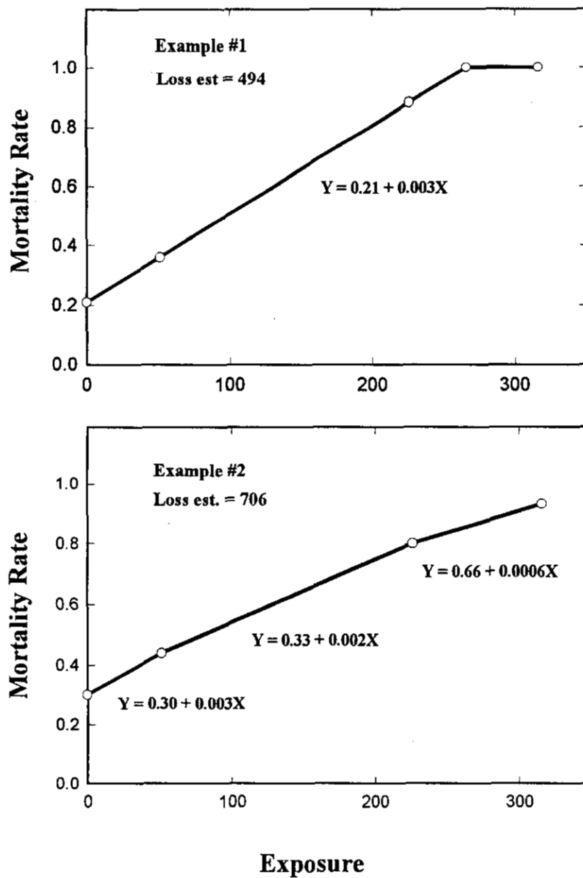
Figure 3. Two examples of the application of exposure dependent mortality rates for the estimation of total acute sea otter mortality along the Kenai Peninsula, Alaska. Exposure measures the number of oil particles that pass within 1.5 km of an observed otter location between 24 March and 23 May 1989.
