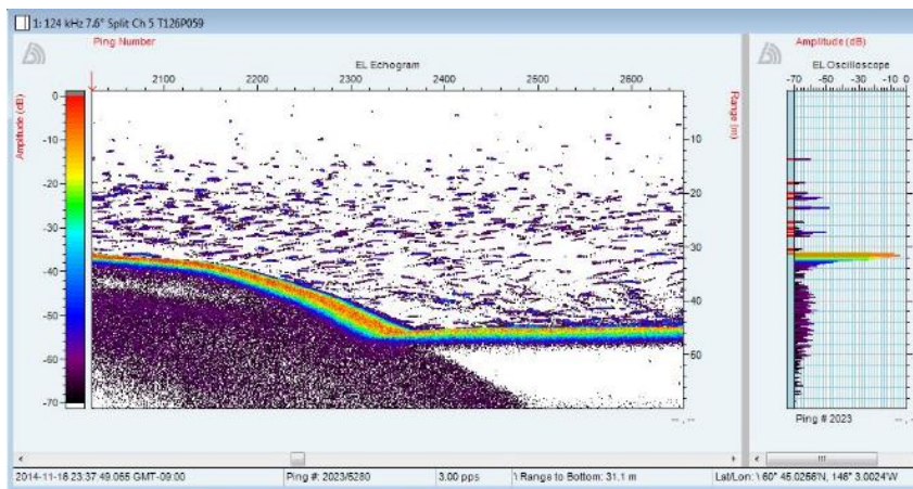
Figure 3. Gravina Bay during trawl 3. This trawl captured 148 herring and 7 capelin.
