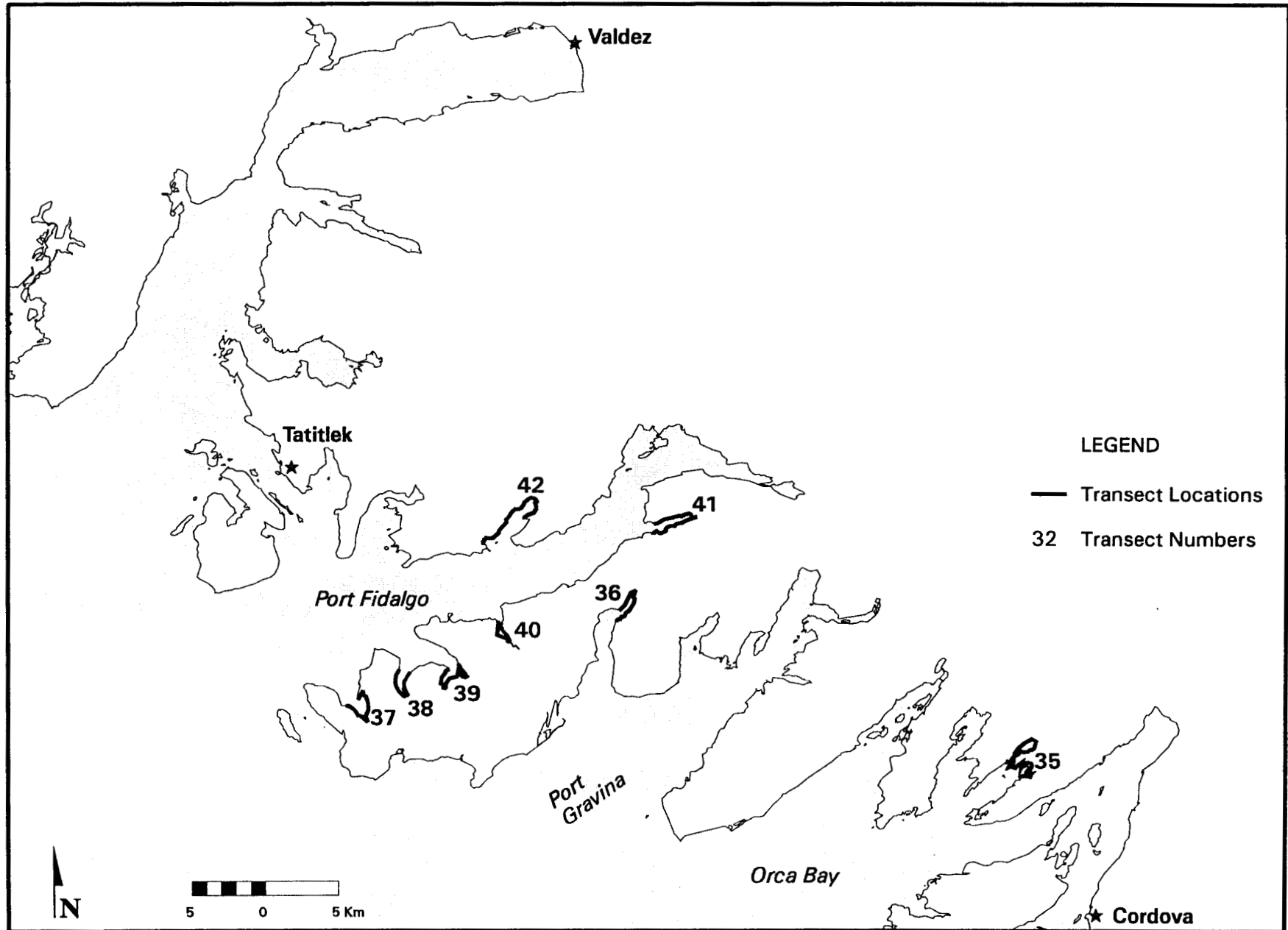
Figure 5. Map of eastern Prince William Sound study area showing the location of transects used during expanded fall surveys in potential brooding rearing areas in 1995 and 1996. Numbers refer to transect numbers listed in tables.
